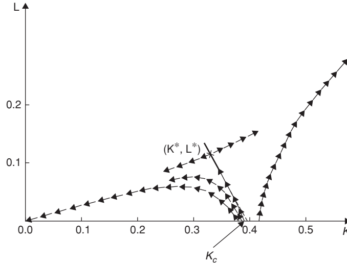
FIGURE 14.6 A section of the critical curve for the two-dimensional Ising model near the nontrivial fixed point ( K^* = \frac{1}{3}, L^* = \frac{1}{9} ). Points on the critical curve flow into the fixed point, while those off it flow away toward the trivial fixed point ( K^* = L^* = 0 ) or ( K^* = L^* = \infty ).
