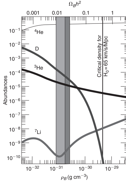
FIGURE 9.4 Calculated primordial abundances of light elements ( {}^4\text{He} , \text{D}={}_1^2\text{H} , {}^3\text{He} , and {}^7\text{Li} ) as functions of the baryon-to-photon ratio. The baryon-to-photon ratio is given by \eta = 2.7 \times 10^{-8} \Omega_b h^2 , where h is the Hubble parameter in units of 100(\text{km/s})/\text{Mpc} and \Omega_b = 0.046 is the current baryonic fraction of the mass-energy density of the universe; see Copi, Schramm, and Turner (1997), Schramm and Turner (1998), and Steigman (2006). The experimentally allowed range is in the grey vertical bands. Figure from Schramm and Turner (1998). Reprinted with permission; copyright © 1998, American Physical Society.
