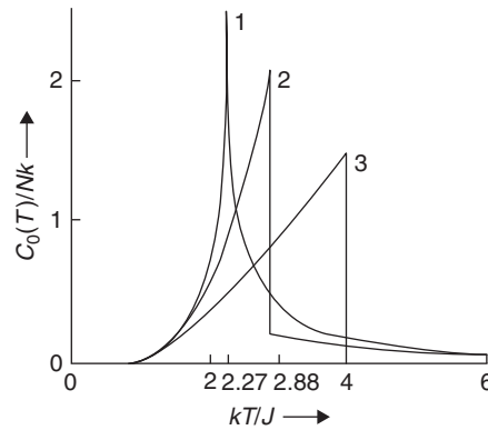
FIGURE 13.14 The specific heat of a square lattice ( q = 4 ) according to (1) the Onsager solution, (2) the Bethe approximation, and (3) the Bragg-Williams approximation.
