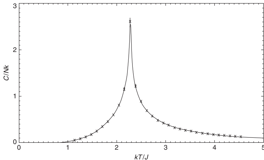
FIGURE 16.1 Monte Carlo specific heat (×'s) of the two-dimensional Ising model on a 128 \times 128 lattice, as compared to the exact solution (solid line) from Section 13.4.A; see Kaufman (1948), Ferdinand and Fisher (1967), and Beale (1996). The MC error bars are smaller than the symbols used, except near the bulk critical temperature T_c(\infty) . Each data point represents an average using 10^5 Monte Carlo sweeps, except at the bulk critical point where 10^6 Monte Carlo sweeps were used to mitigate critical slowing down.
