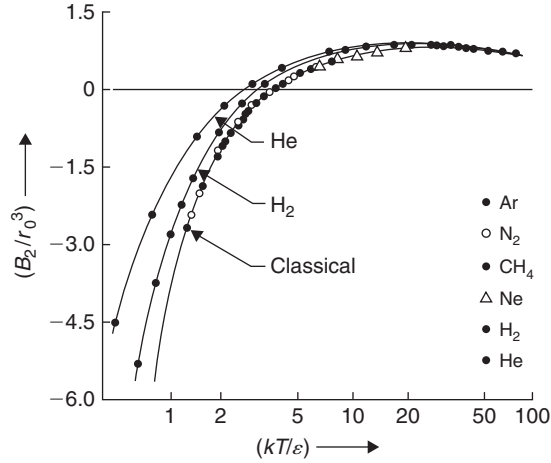
FIGURE 10.2 A dimensionless plot showing the temperature dependence of the second virial coefficient of several gases (after Hirschfelder et al., 1954).
