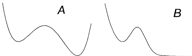
Figure 4.2.1 Potential energy as a function of reaction coordinate in two typical cases, A is a potential with two minima, and B is a potential that allows escape from a single minimum.
