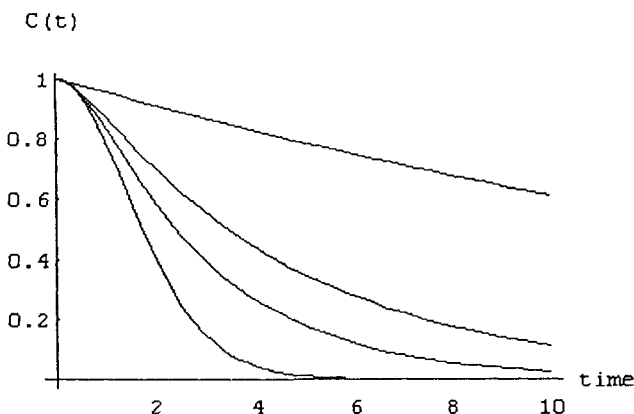
Figure 5.2.1 Results of numerical inversion of the Laplace transform of the orientational time correlation function. The relaxation time \tau takes the values 10 (lowest curve), 1, 0.5, and 0.1 (highest curve).
